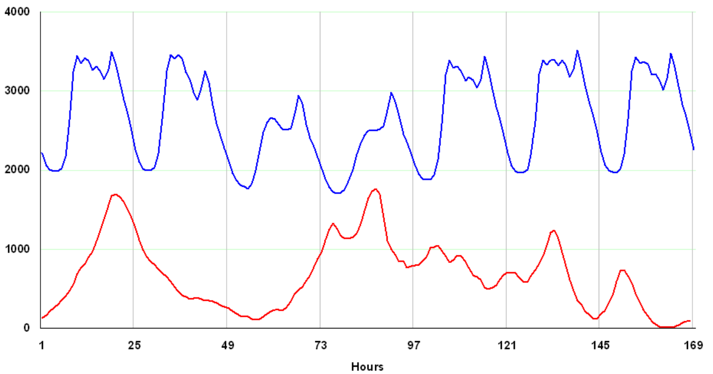
West Denmark - Jan 8 to 14 2004 - Consumption versus Wind Production
