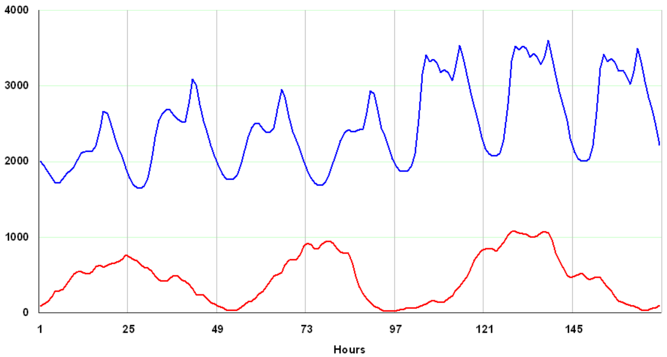
West Denmark - Jan 1 to 7 2004 - Consumption versus Wind Production
