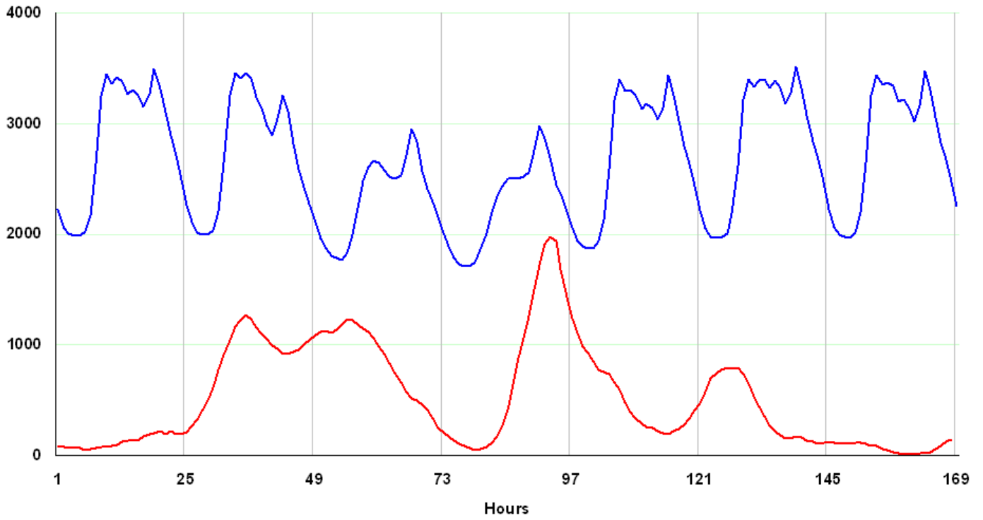
West Denmark - Jan 15 to 21 2004 - Consumption versus Wind Production
