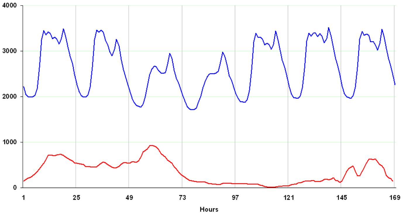
West Denmark - Jan 22 to 28 2004 - Consumption versus Wind Production
