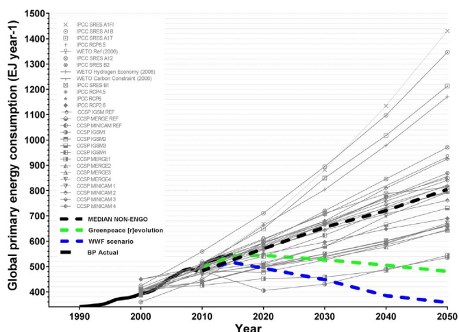
Fig. 1. Comparison of scenarios for global primary energy from the Intergovernmental Panel on Climate Change (IPCC), the Climate Change Science Program (CCSP), the World Energy Technology Organisation (WETO), the BP Statistical Review, Greenpeace and the World Wildlife Fund (WWF). Sources: US Energy Information Administration (EIA) [59]; Intergovernmental Panel on Climate Change [105]; Jeffries et al. [108] Teske et al. [15]; European Commission [106], Van Vuuren et al. [109]. All WETO values are converted from million tonnes oil-equivalent. All EIA values are converted from quadrillion British Thermal Units. Greenpeace values are converted from petajoules. All WWF values were published as final energy only and are converted from final energy to primary energy based on the ratio of primary to final energy provided in the Greenpeace scenario.
