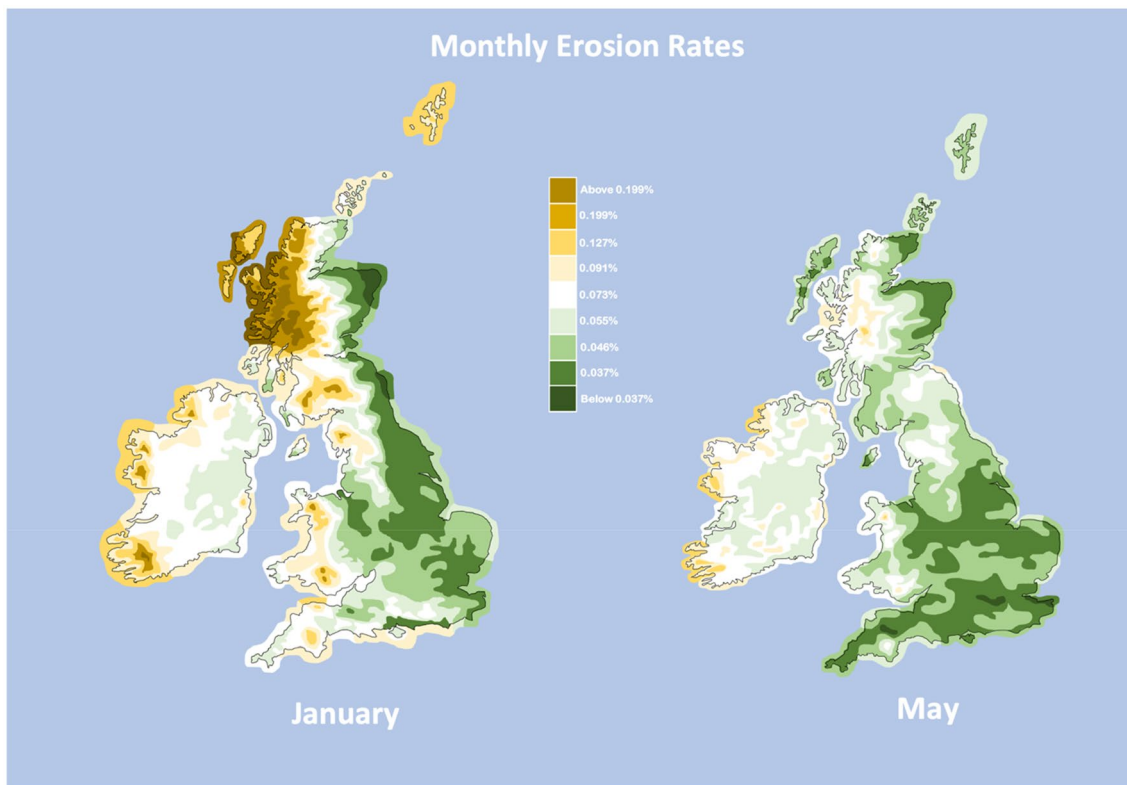
Fig. 4 The monthly erosion rates of the tip of a turbine blade along the leading edge in January and May
