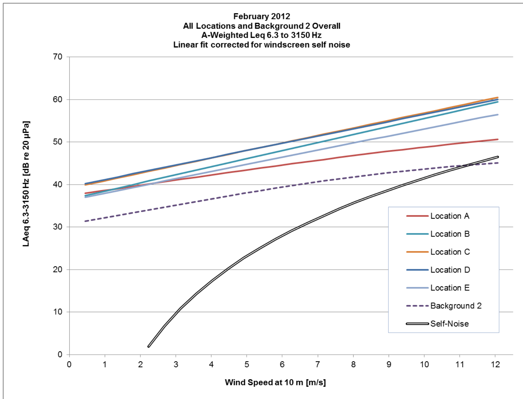
Figure C54. All locations and Background 2 Overall A-weighted Leq 6.3 to 3150 Hz linear fit corrected for windscreen self-noise.
