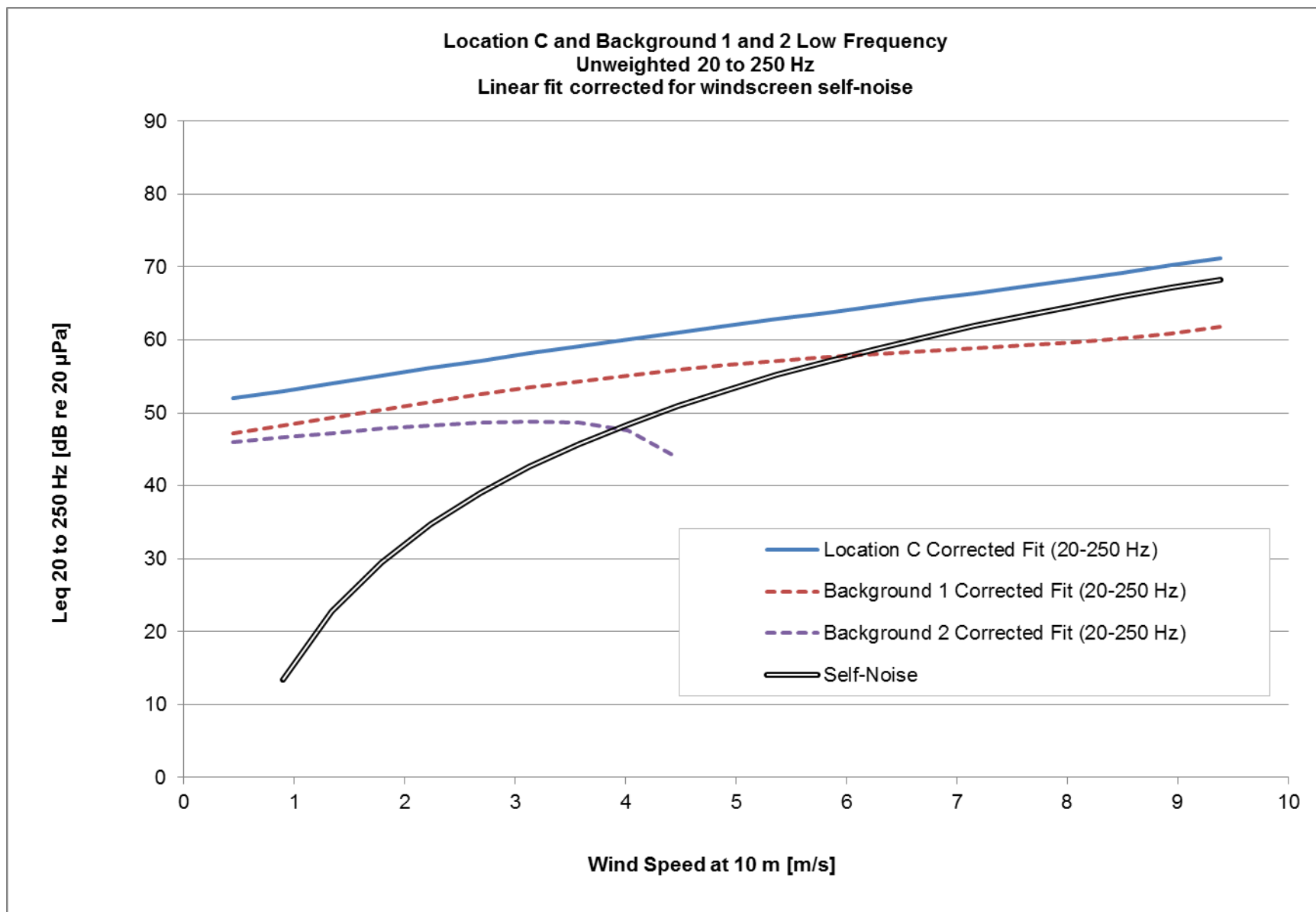
Figure C28. Location C and Background 1 and 2 low frequency unweighted 20 to 250 Hz linear fit corrected for windscreen self-noise.
