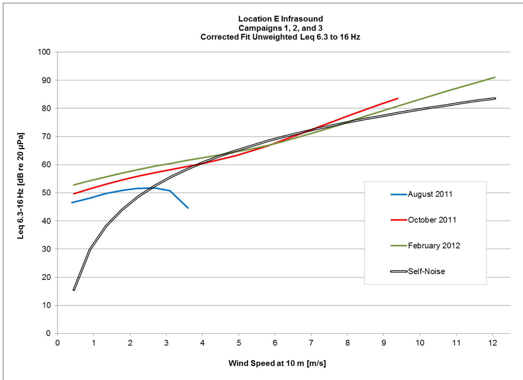
Figure C58. Location E Infrasound Campaigns 1, 2, and 3 corrected fit unweighted Leq 6.3 to 16 Hz.
