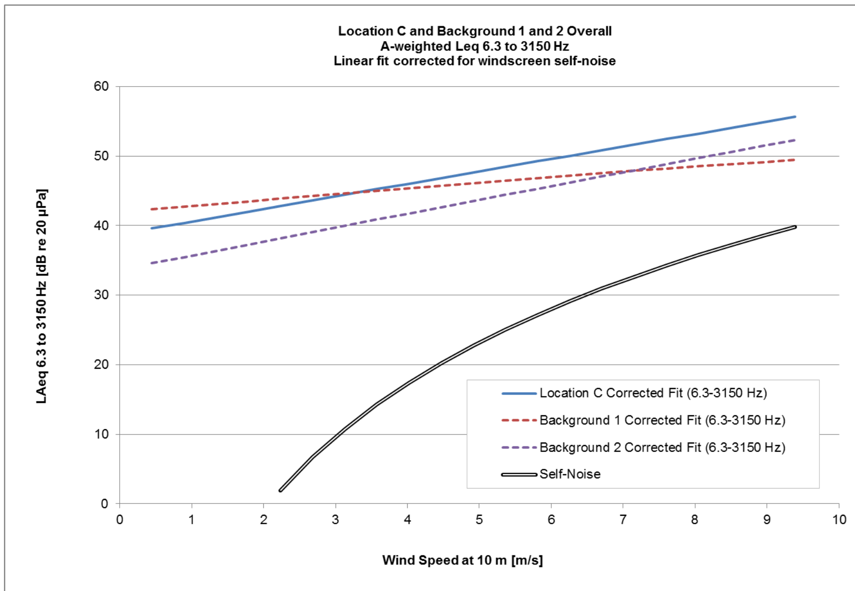
Figure C33. Location C and Background 1 and 2 overall A-weighted Leq 6.3 to 3150 Hz linear fit corrected for windscreen self-noise.
