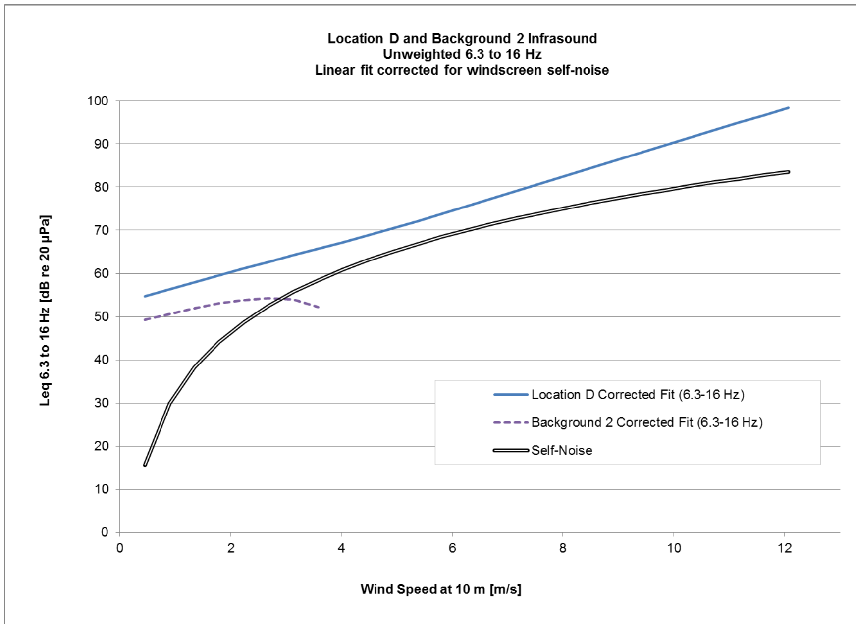
Figure C40. Location D and Background 2 Infrasound Unweighted 6.3 to 16 Hz linear fit corrected for windscreen self-noise.
