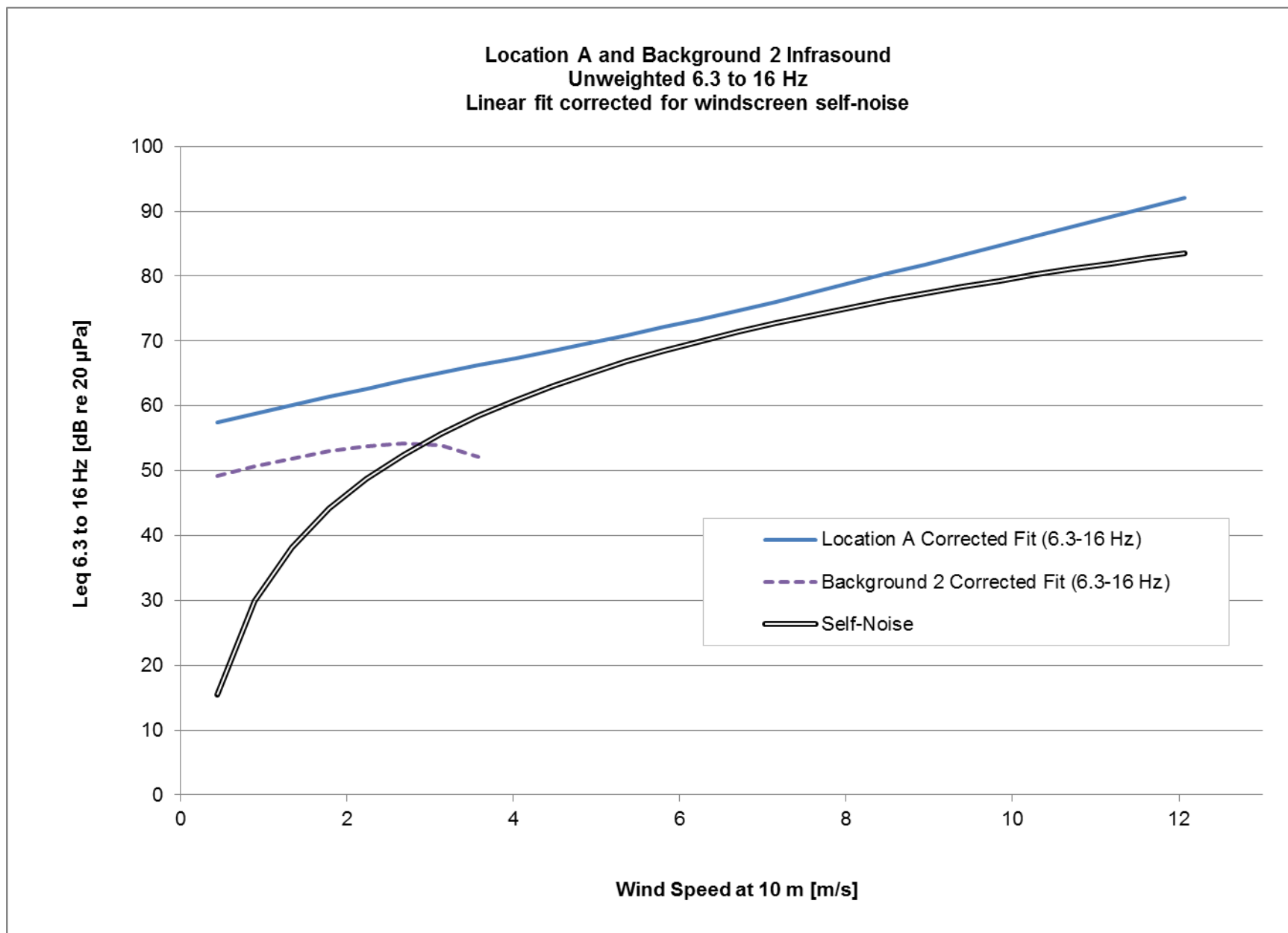
Figure C37. Location A and Background 2 Infrasound Unweighted 6.3 to 16 Hz linear fit corrected for windscreen self-noise.
