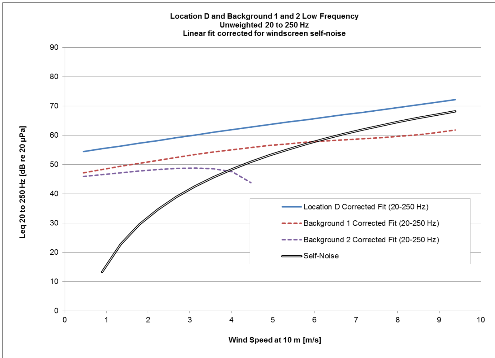
Figure C29. Location D and Background 1 and 2 low frequency unweighted 20 to 250 Hz linear fit corrected for windscreen self-noise.
