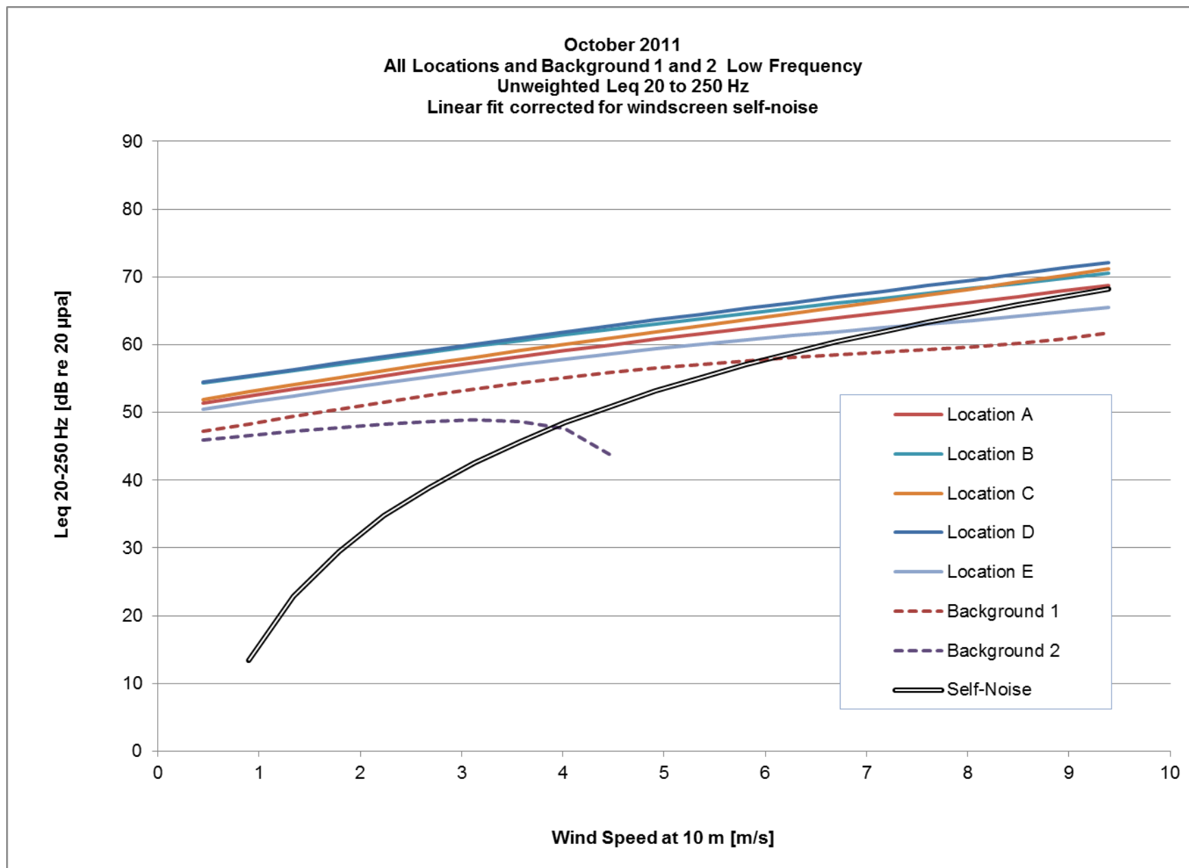
Figure C30. All Locations and Background 1 and 2 low frequency unweighted 20 to 250 Hz linear fit corrected for windscreen self-noise.
