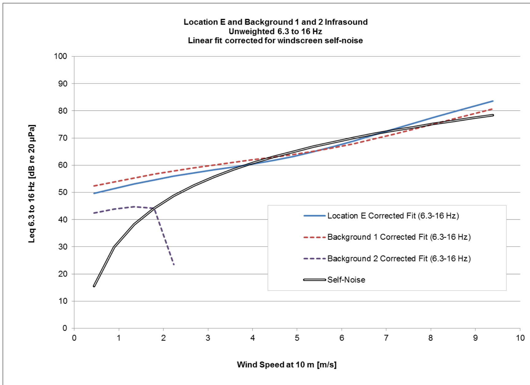
Figure C19. Location E and Background 1 and 2 Infrasound unweighted 6.3 to 16 Hz linear fit corrected for windscreen self-noise.
