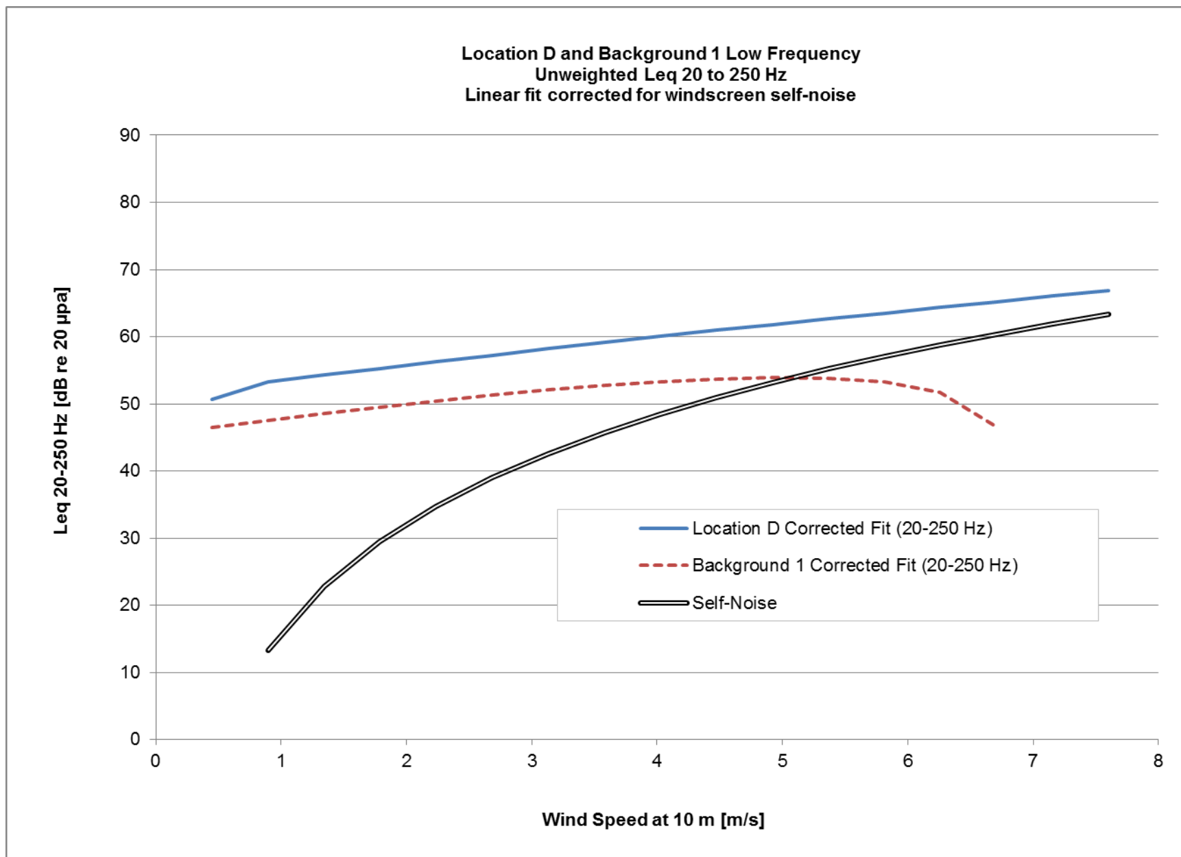
Figure C8. Location D and Background 1 Low frequency unweighted Leq 20 to 250 Hz linear fit corrected for windscreen self-noise.
