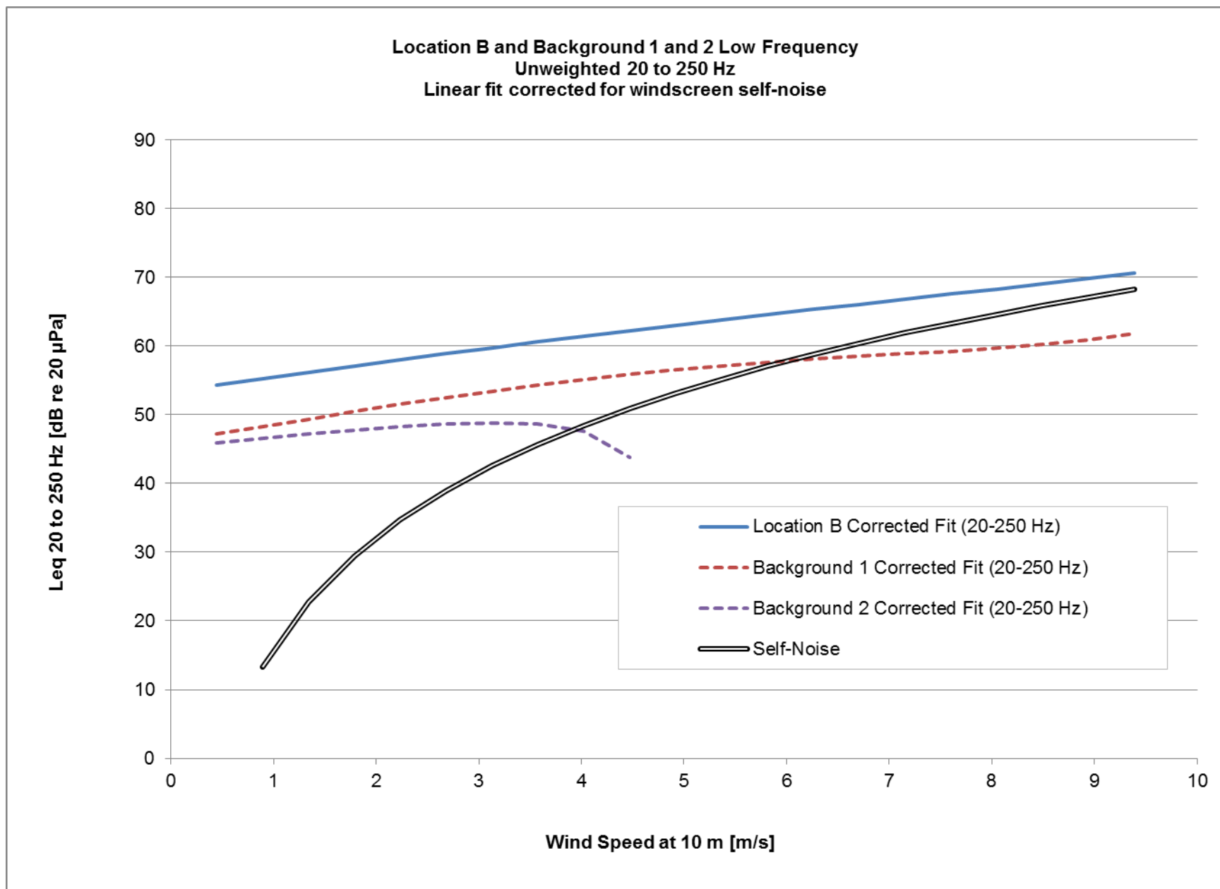
Figure C27. Location B and Background 1 and 2 low frequency unweighted 20 to 250 Hz linear fit corrected for windscreen self-noise.
