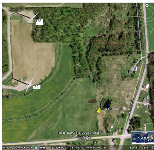
Figure 2. Monitoring Location B with respect to the nearest wind turbines.
