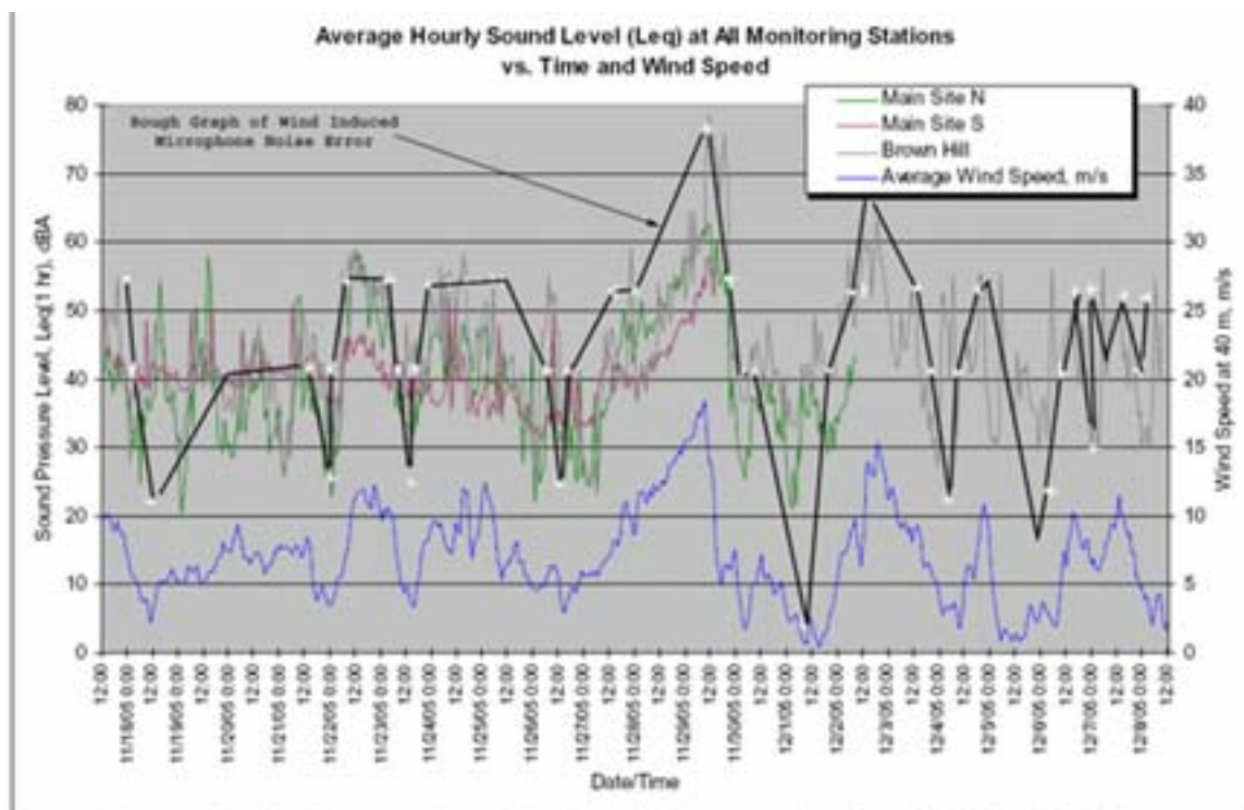
Figure 2.5.2 Hourly Average Sound Levels at All Positions vs. Wind Speed (11/17 to 12/8/05)
