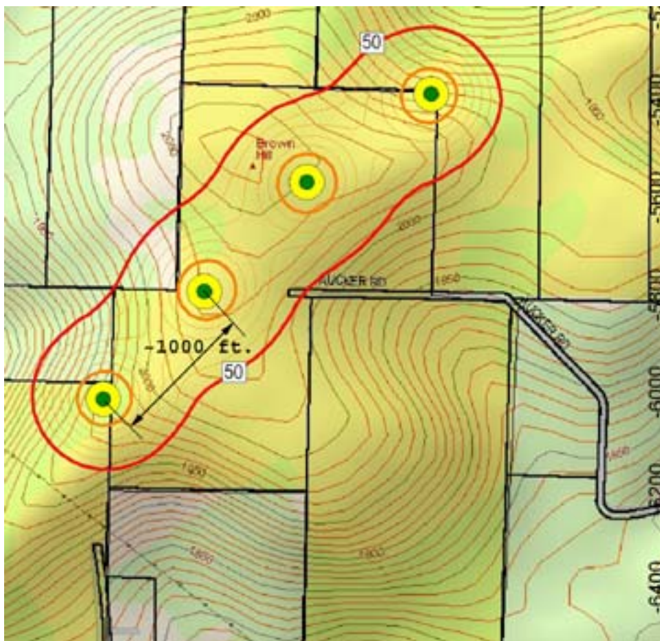
Fig. 9: Enlarged View of Graphic C, Hessler Predicted Noise Contours with Light Omnidirectional Wind
