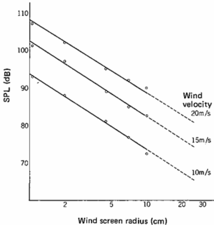
Fig 6: Relation between wind screen size and wind noise (Ref. 4)
