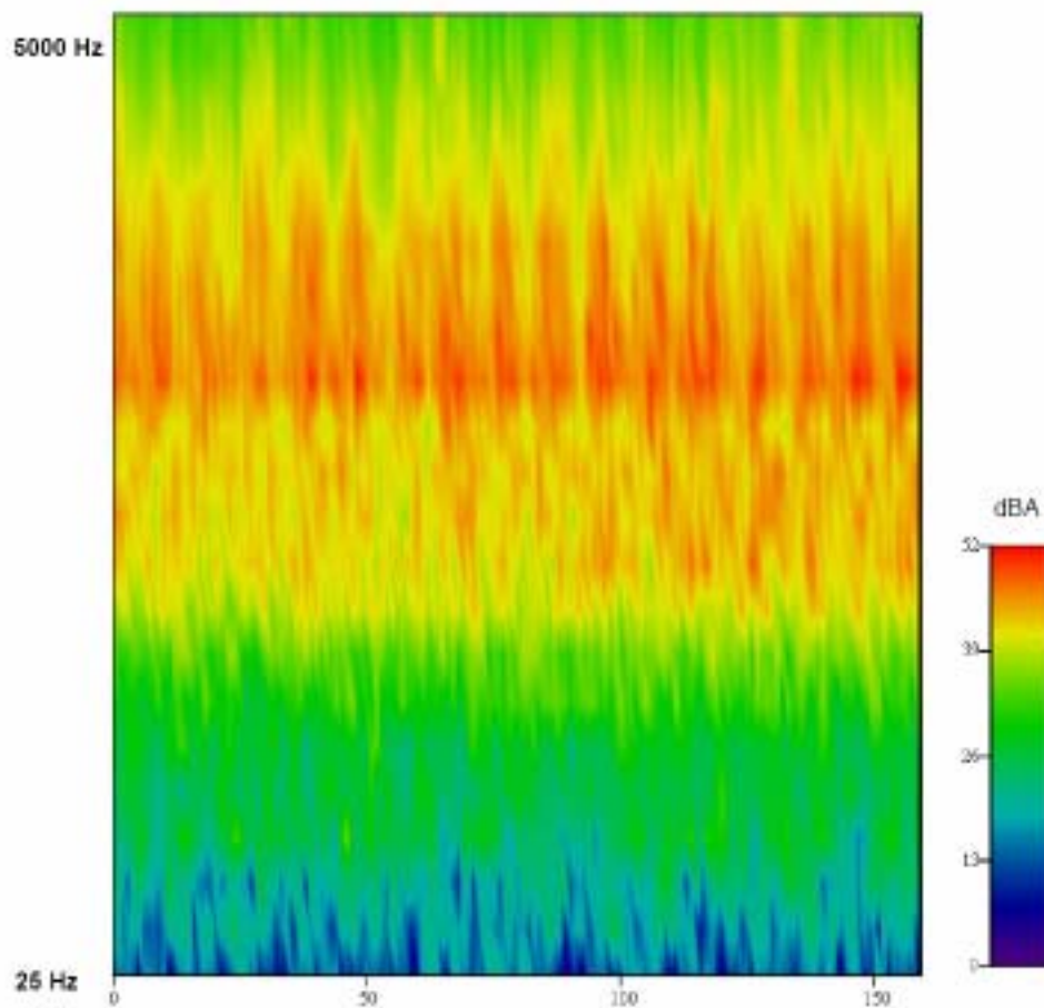
Fig. 13: Sample Spectrum of Noise Modulation (Pubnico Point, ob cit )
