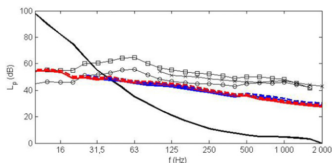
Figure 1. 1/3 octave sound power level spectra from old turbines <2 MW (—) and new \geq 2 MW (---), recalculated from Madsen and Pedersen (2010) to an average level of 40 dB ( L_{Aeq} ) at 500 m distance (solid) and 1000 m distance (dashed). For comparison, ISO717-1 (ISO 717-1 1996a) spectra for road traffic noise (x), measured road traffic noise 10 m distance (o) (light traffic) and recalculated at 500 m (□) are shown at 55 dB ( L_{Aeq} ), as well as the absolute detection threshold (—) (Watanabe and Møller 1990).
